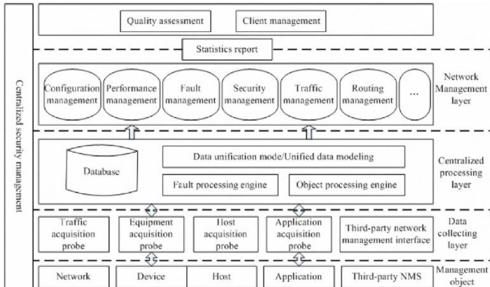
Figure 1. Structure of Network Management System
