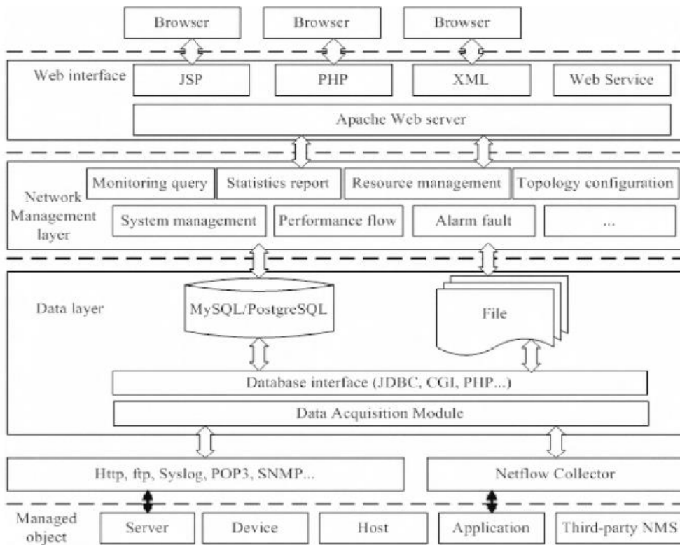
Figure 4. Structure of NMS technology
