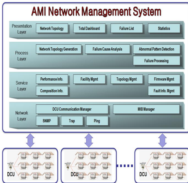
Fig. 3. Layered architecture of AMI Network Management System.
