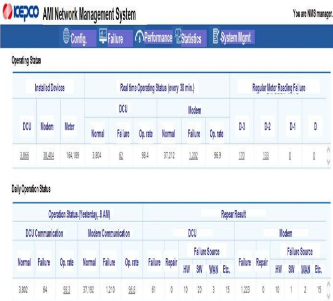
Fig. 7. Web-based total dashboard screen of AMI NMS.
